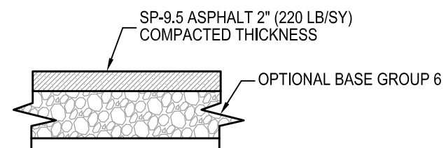
TYPICAL SECTION ROADWAY TURNOUT CONSTRUCTION DETAIL
