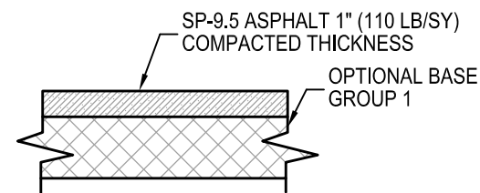
TYPICAL SECTION DRIVEWAY TURNOUT CONSTRUCTION DETAIL
