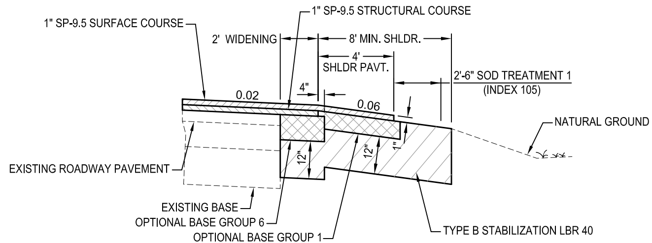
TYPICAL SECTION WIDENING DETAIL
